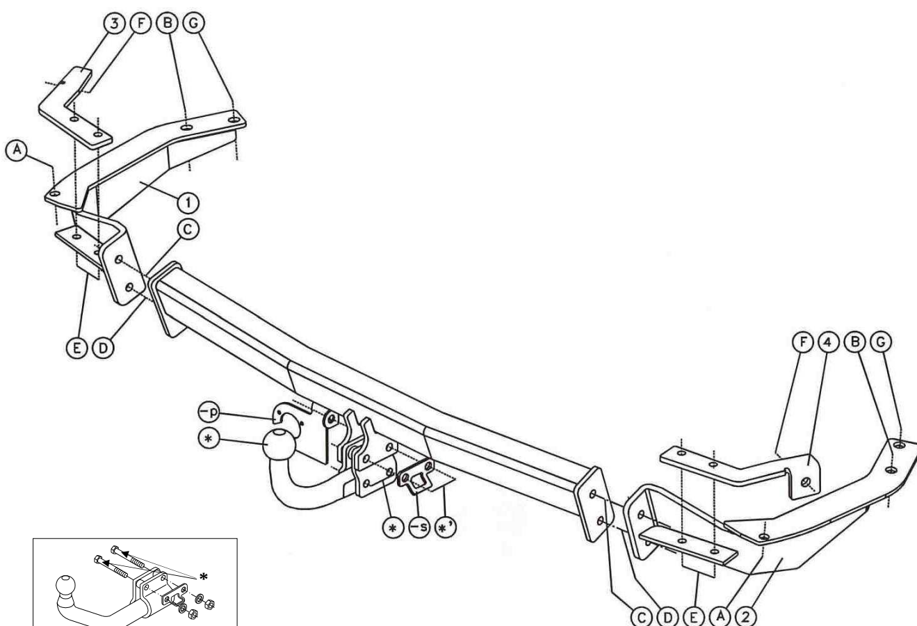
Montering af fast kulestang system T45
